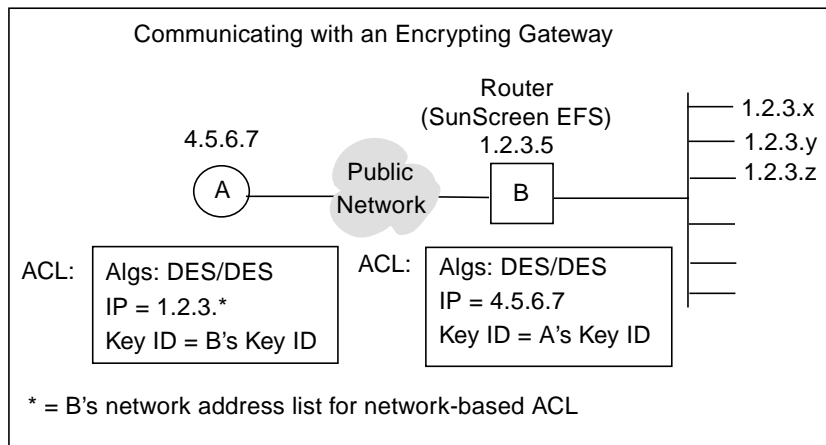
FIGURE 5-3 Communicating with an Encrypting Gateway
