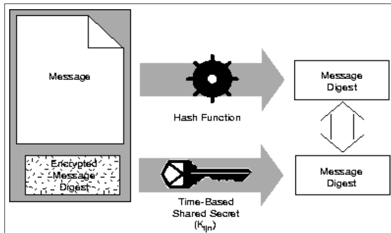
FIGURE B-8 Authenticating a Message
